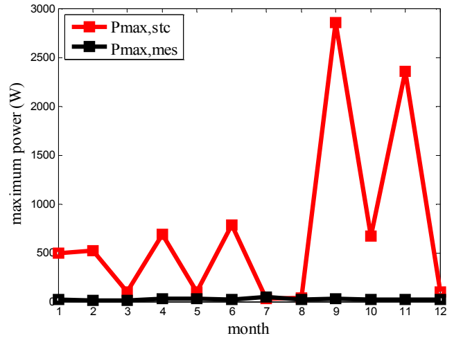
Figure 4. Curve of maximal power measured (black) and translate (red) obtained with Bleasser's method.
