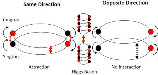
Fig. 5. Gravitational Force between two Higgs Bosons.
